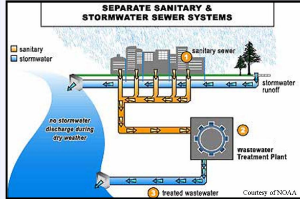
Separate storm and sanitary sewer systems
