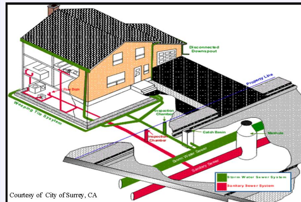
Red is sanitary, green is storm—lot level detail
